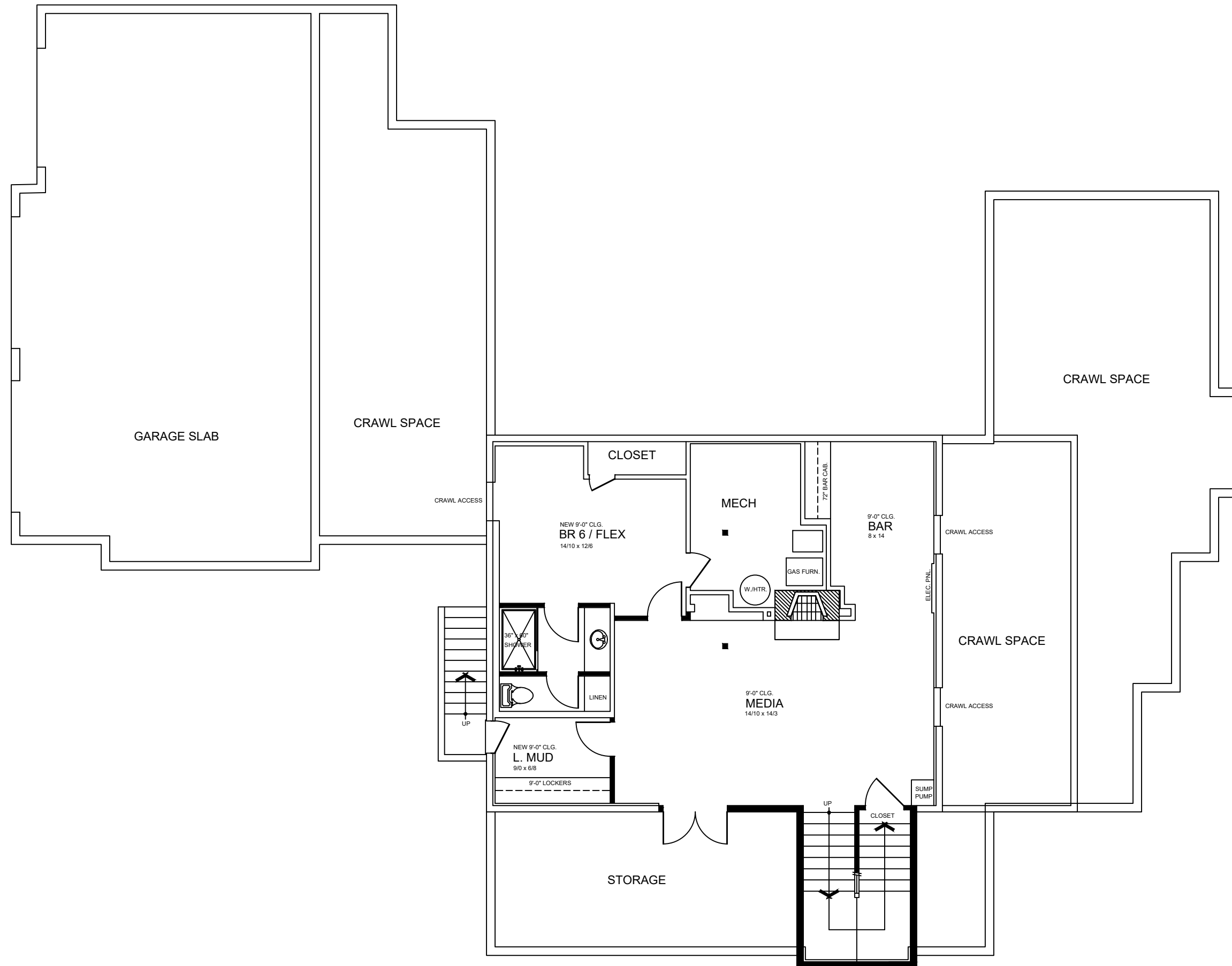
LOWER LEVEL FLOOR PLAN 1,200 SF
