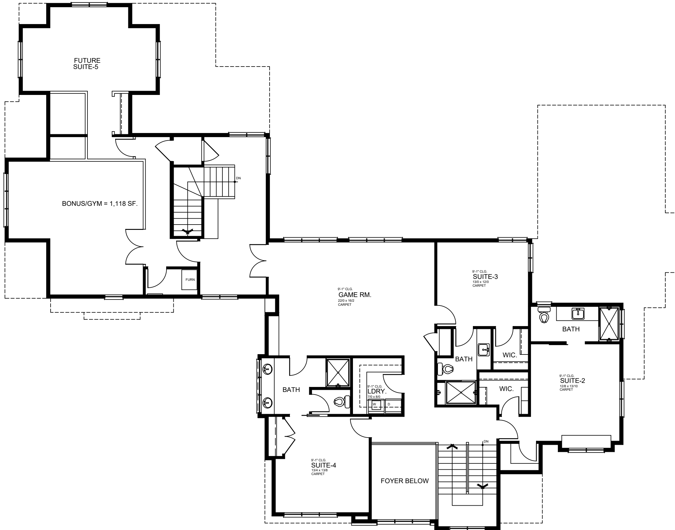
SECOND FLOOR PLAN 1,554 SF
